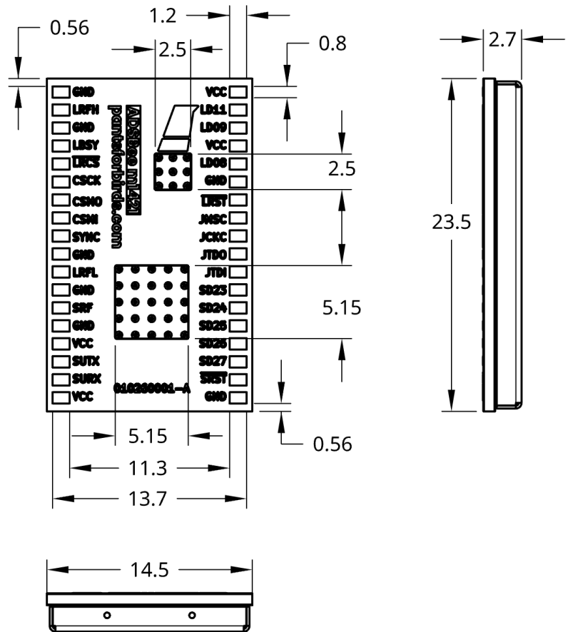
BOTTOM VIEW
