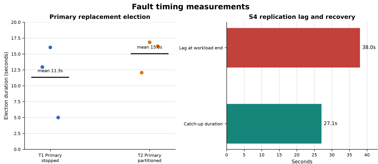
Figure 5. Primary-replacement election durations for T1/T2 (three seeds per scenario), together with S4 replication-lag and catch-up durations.
