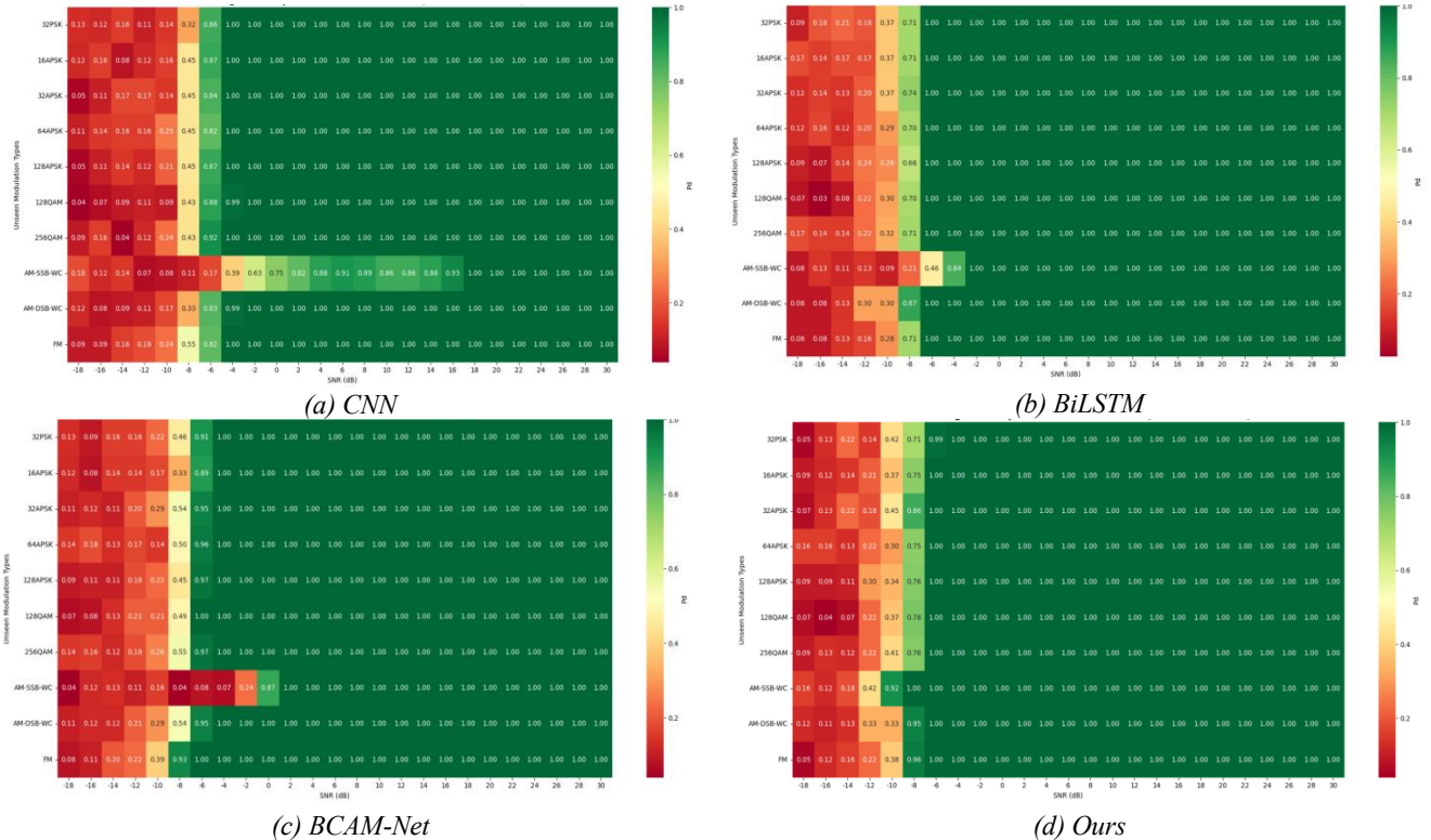
Fig. 4. Modulation-wise detection probability P_d heatmaps on Test Set 2 for unseen modulation formats: (a) CNN, (b) BiLSTM, (c) BCAM-Net, and (d) the proposed method. All panels use identical modulation and SNR orders, a shared color scale, and thresholds calibrated on the corresponding validation sets.
