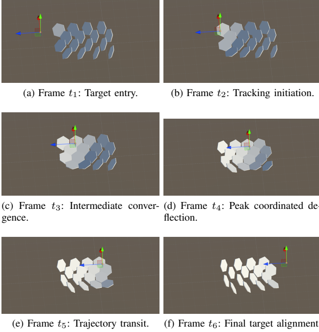
Fig. 1. Simulation sequence of the 16-module SOFIA honeycomb array tracking a dynamic 3D target point. (a)–(c) Target enters the system workspace, prompting orientation convergence across proximal modules. (d)–(f) Synchronized multi-unit re-orientation maintaining normal vector \hat{\mathbf{r}}_{2,3} alignment toward \mathbf{p}(t) under actuator saturation constraints.
