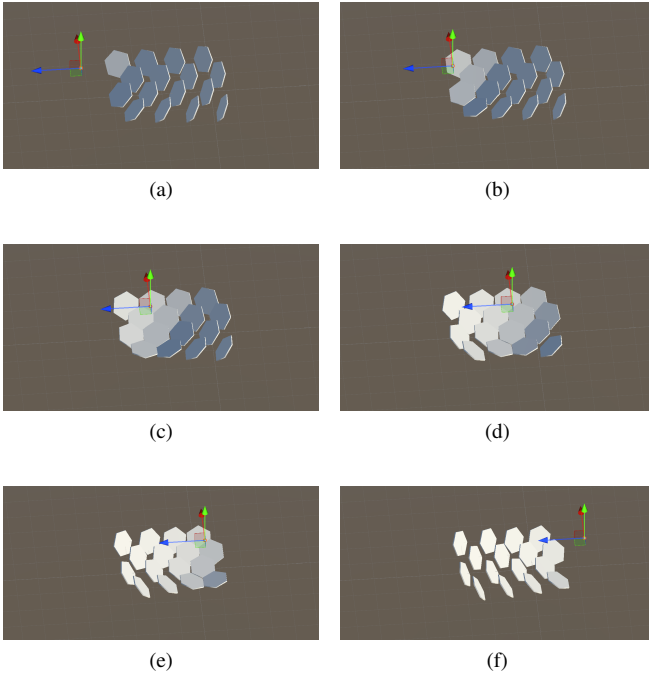
Fig. 1. Representative frames of the SOFIA kinematic tracking simulation. The six frames illustrate the progressive reorientation of the 16-module honeycomb array as the target coordinate \mathbf{p}(t) moves through the workspace, with the module normal vectors \hat{\mathbf{r}}_{2,3}^{(i)} oriented toward the target.
