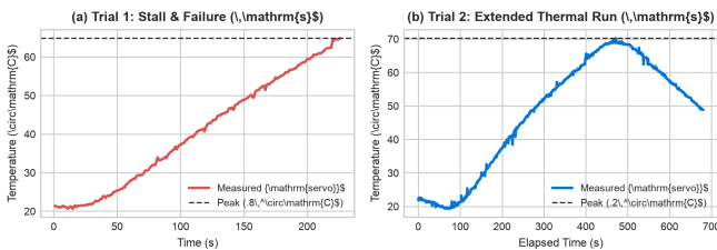
Fig. 1. Experimental thermal characterization of the MG90S servomotor under persistent mechanical stall: (a) Trial 1 heating curve until audible failure at t = 226 \text{ s} ( T_{\max} = 64.84^\circ\text{C} ); (b) Trial 2 extended thermal cycle across 682 data points reaching peak steady-state temperature of 70.21^\circ\text{C} .
