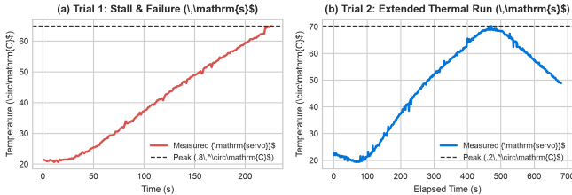
Fig. 1. Experimental thermal characterization of the MG90S servomotor under persistent mechanical stall: (a) Trial 1 heating curve until audible failure at t = 226 \text{ s} ( T_{\max} = 64.84^\circ\text{C} ); (b) Trial 2 extended thermal cycle across 682 data points reaching peak steady-state temperature of 70.21^\circ\text{C} .
