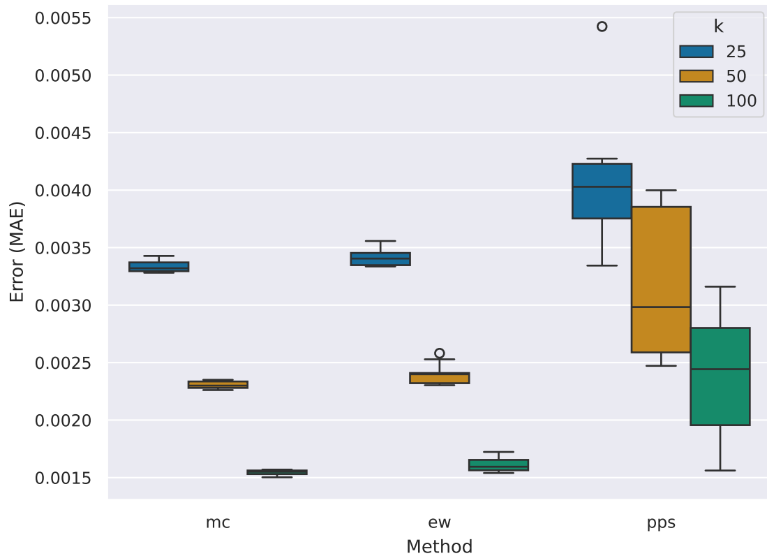
Error Over k
