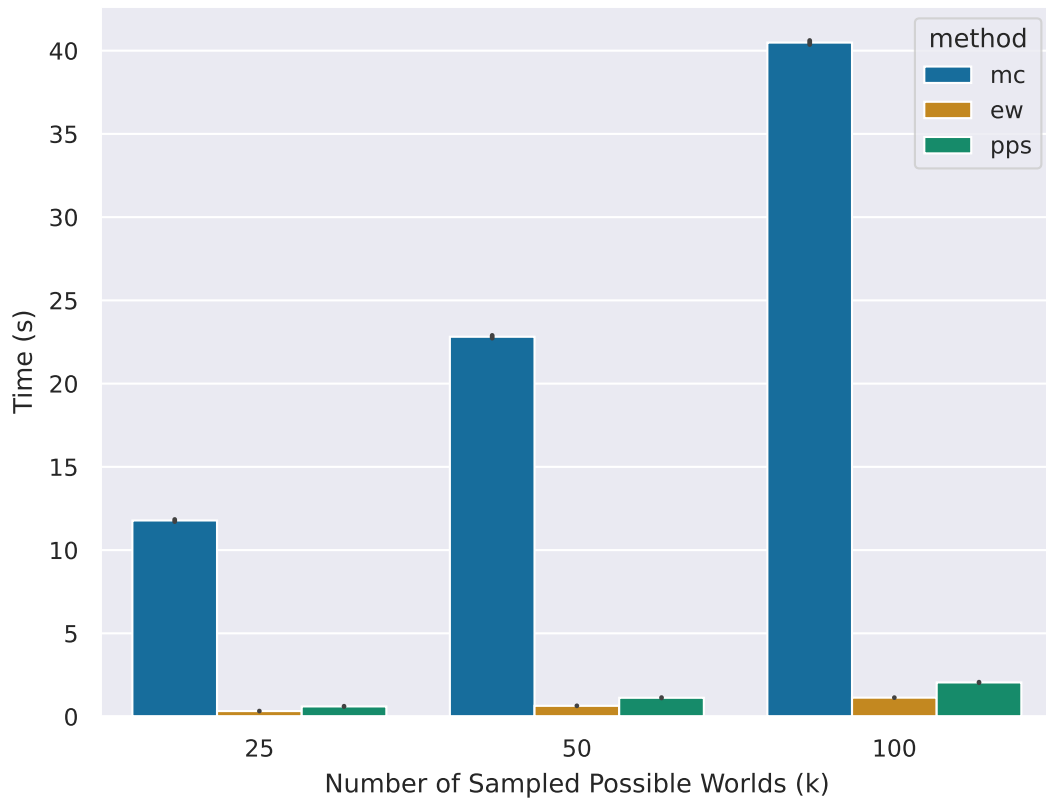
Running Time Over k
