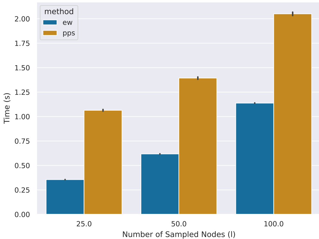
Running Time Over I
