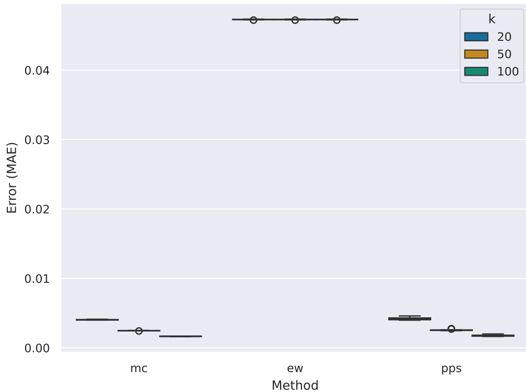
Error Over k
