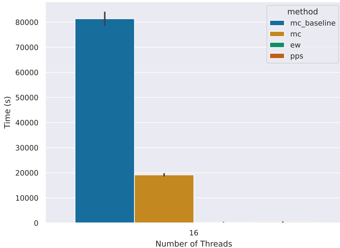
Running Time Over Threads
