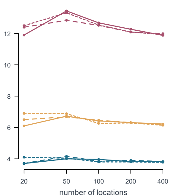
mean degree
