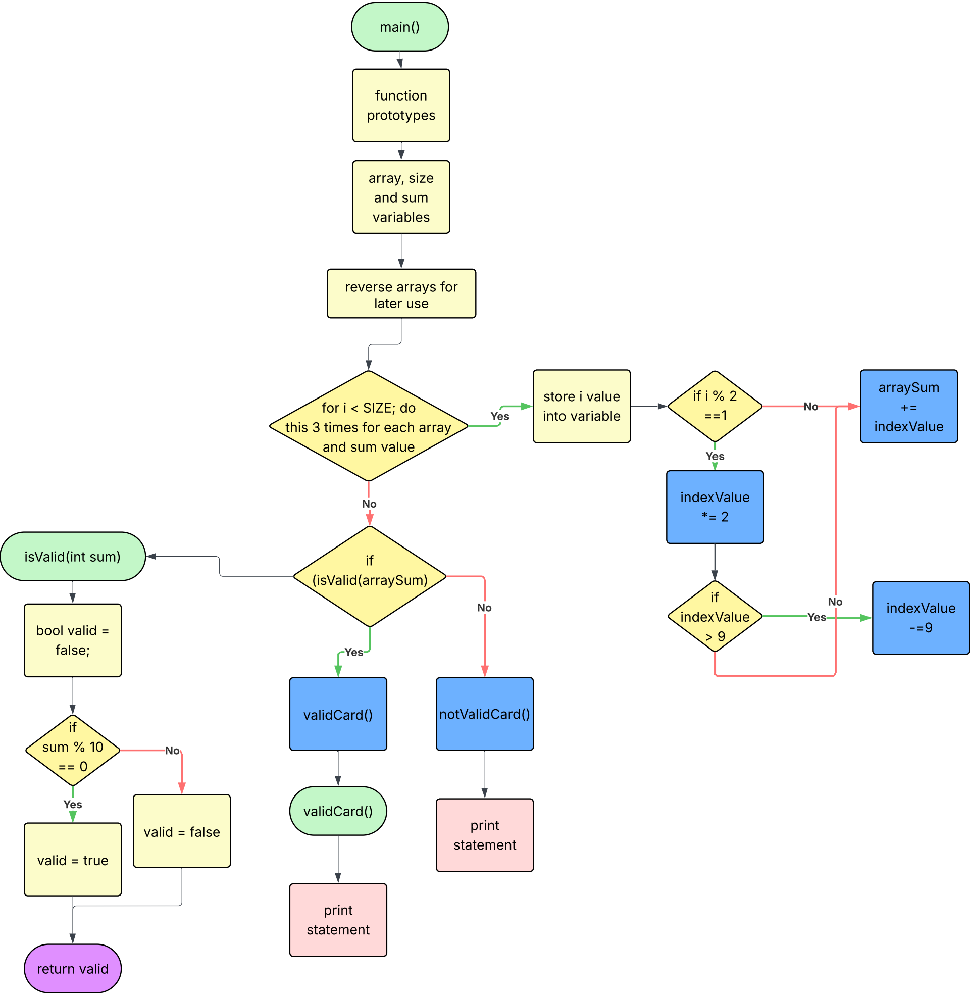
Luhn_Algorithm
