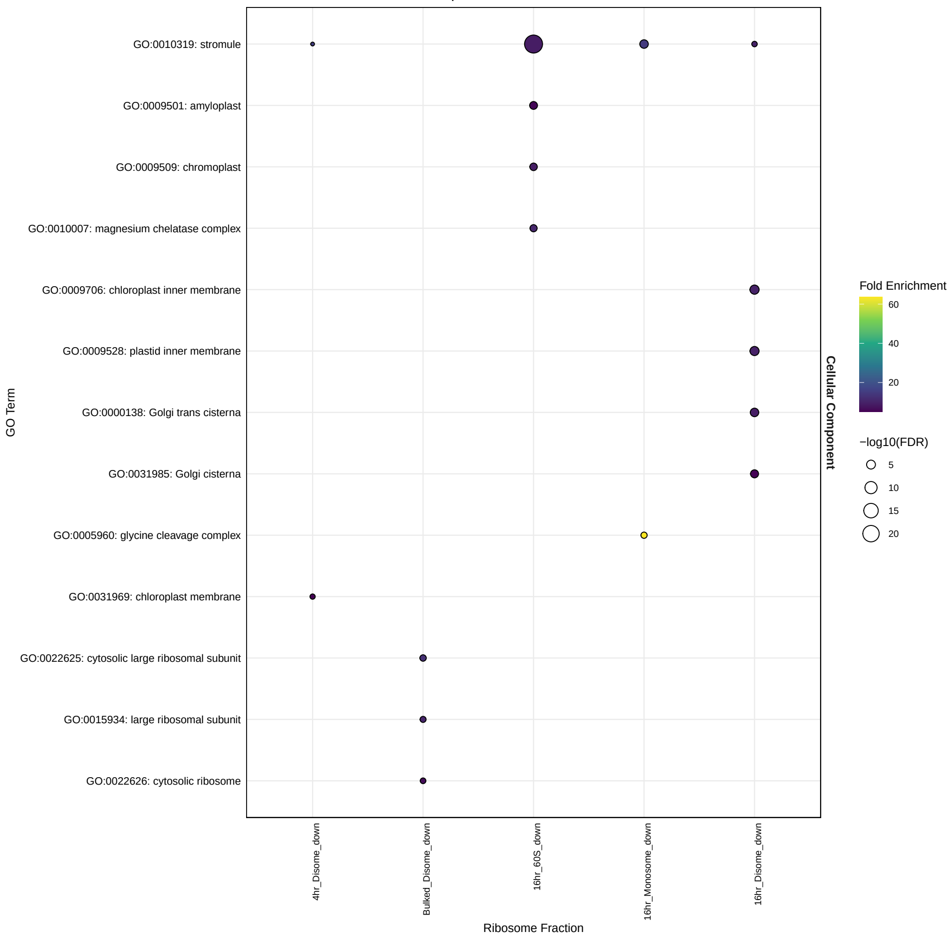
DOWN Clusters – Cellular Component
