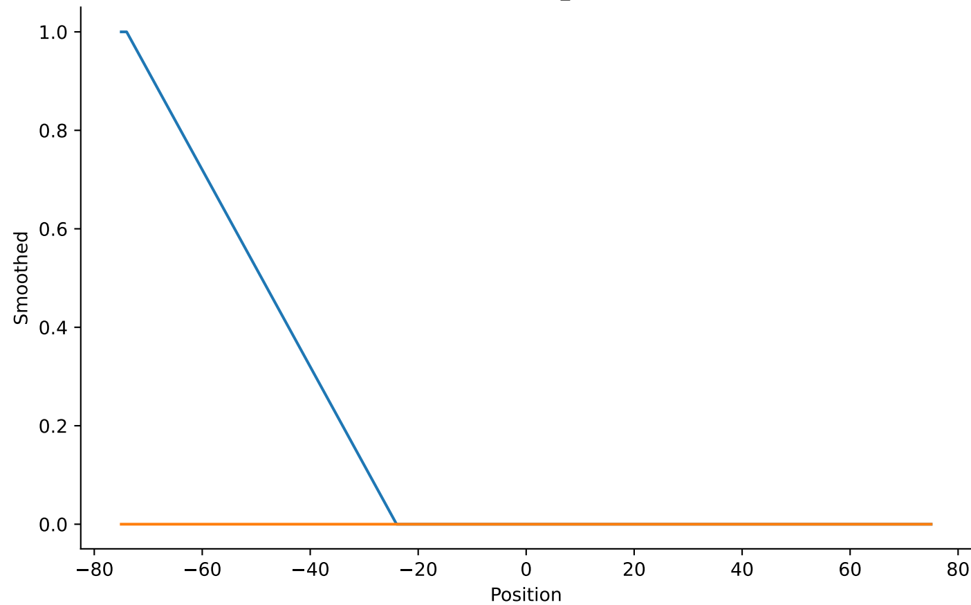
Anchor = Start_Codon
