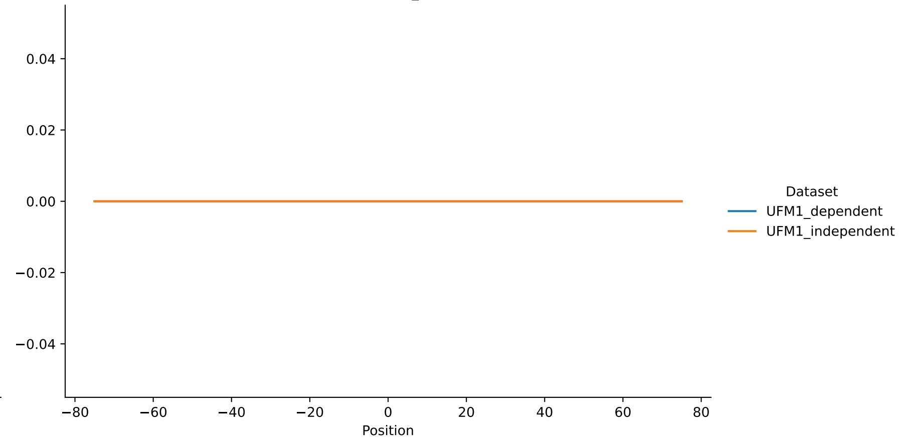
Anchor = Stop_Codon
