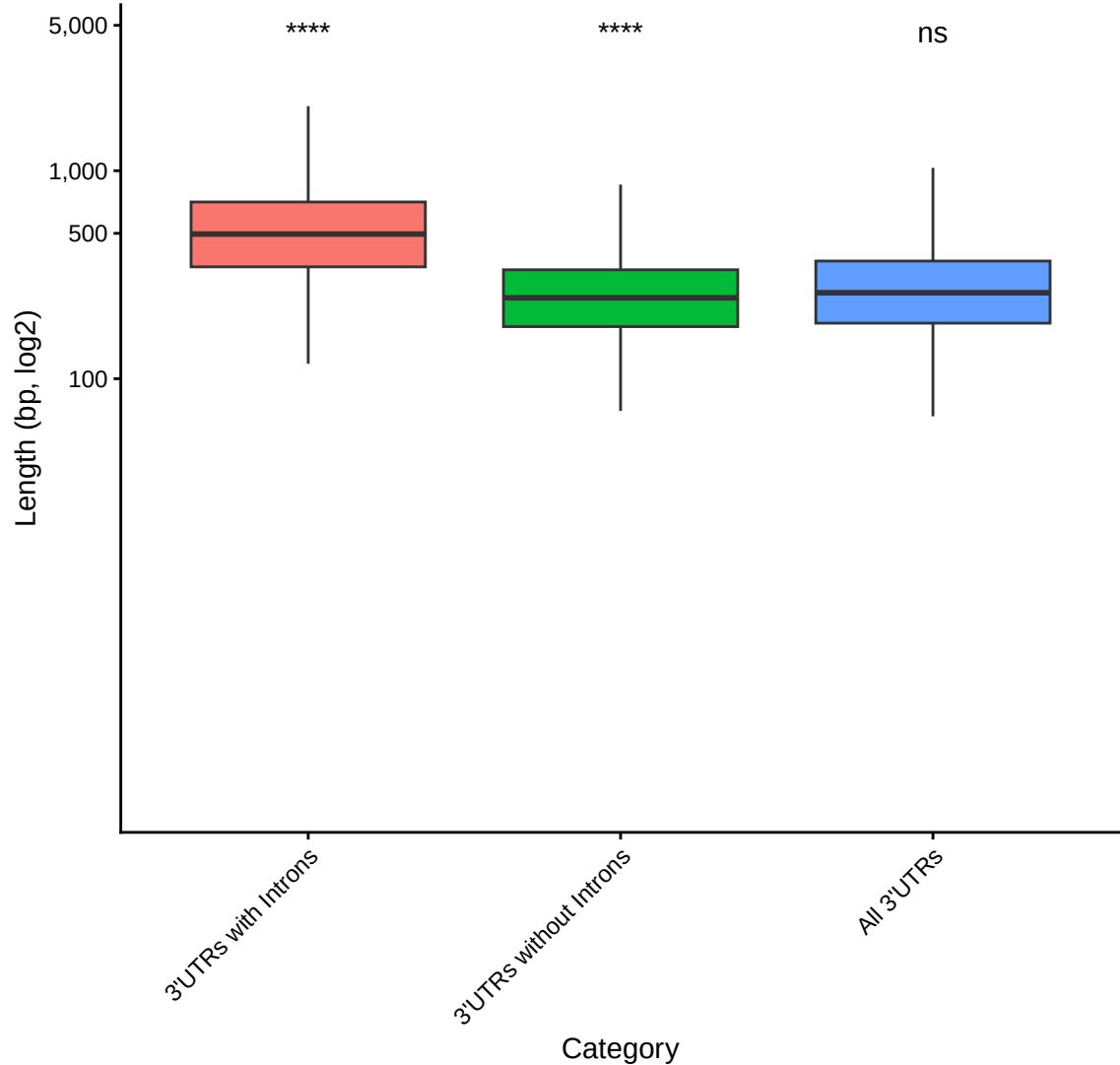
3'UTR Length Distribution
