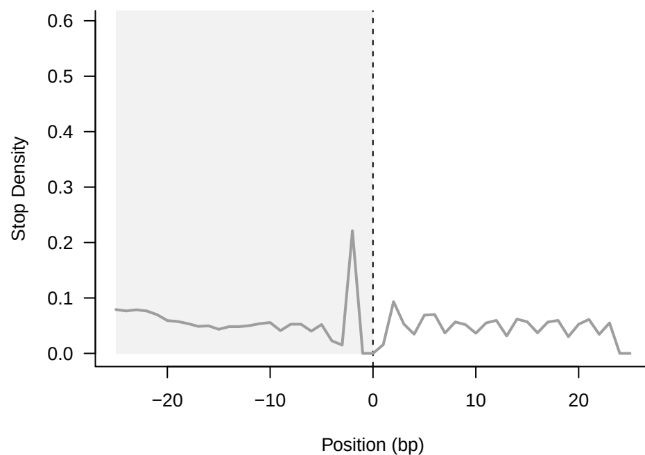
D. Stop Codons: 3' Anchored
