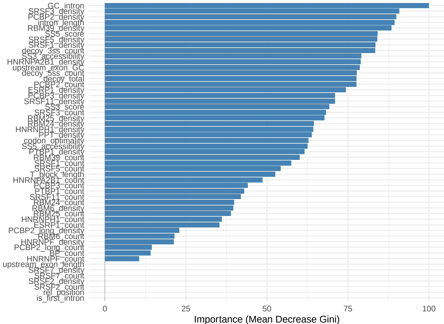
Variable Importance: UFM1-Dependent vs Independent
