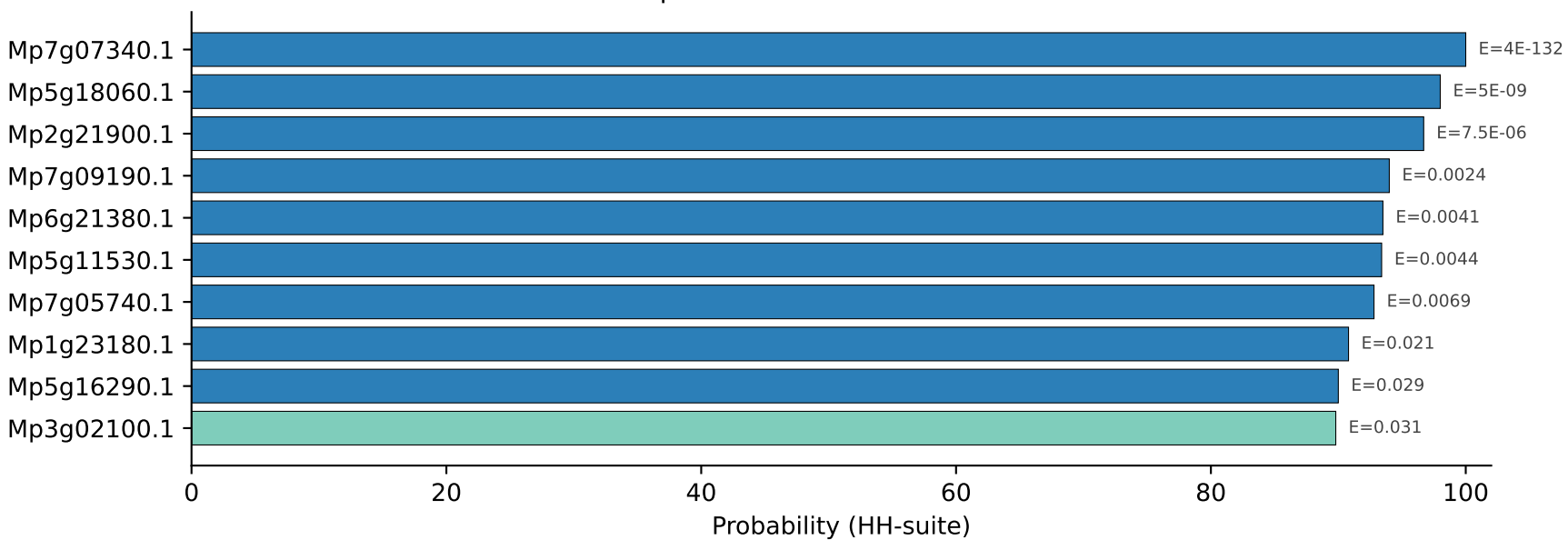
Top 10 Marchantia hits for LTN1
