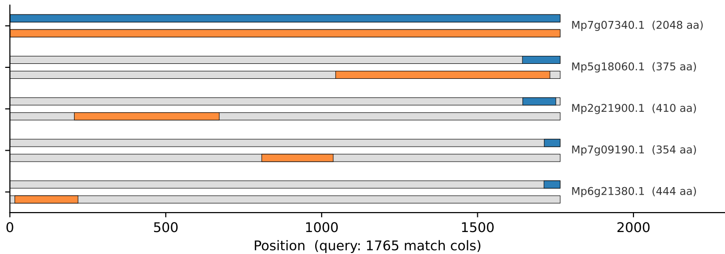
Coverage: query (blue, top) vs template (orange, bottom) — top 5
