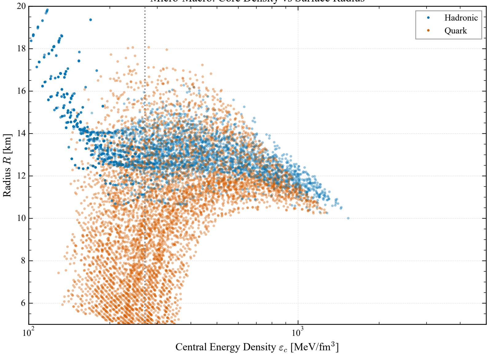
Micro-Macro: Core Density vs Surface Radius
