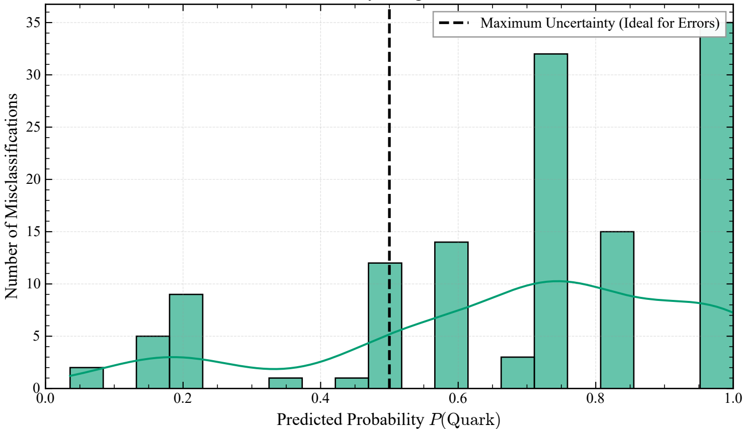
Calibration Check: Probability Assigned to Incorrect Predictions
