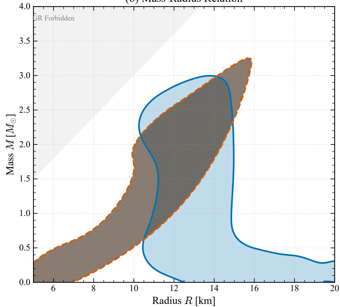
(b) Mass-Radius Relation
