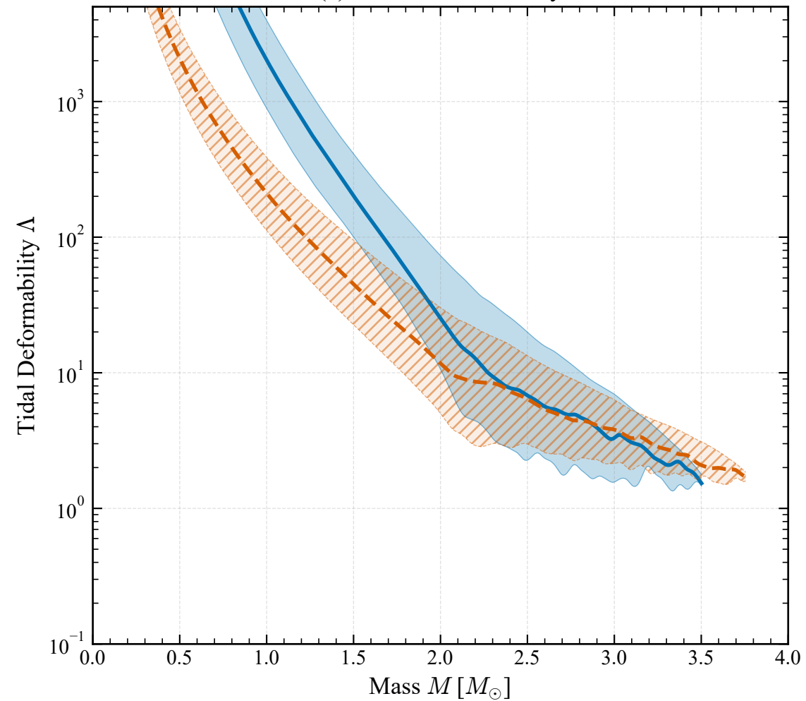
(c) Tidal Deformability
