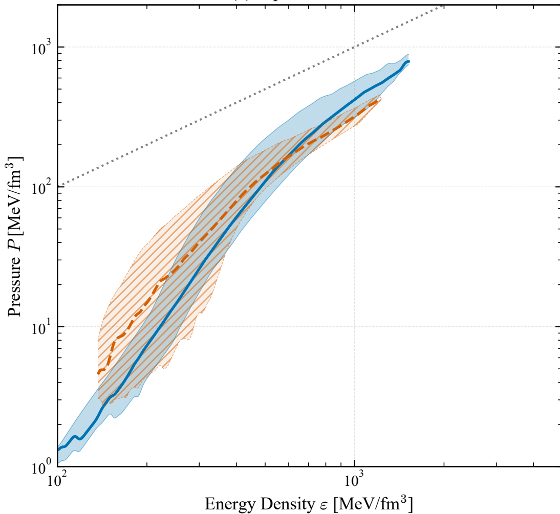
(a) Equation of State
