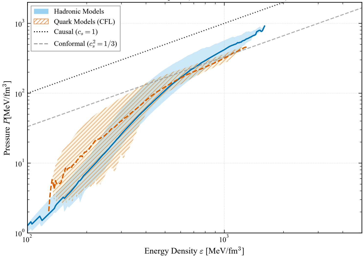
Prior EoS Phase Space (90% Confidence Intervals)
