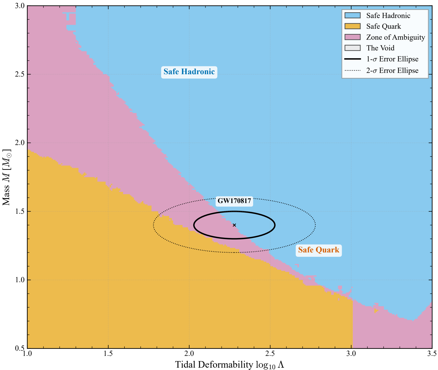
Model A: Resolving Degeneracy with \Lambda (Ensemble)
