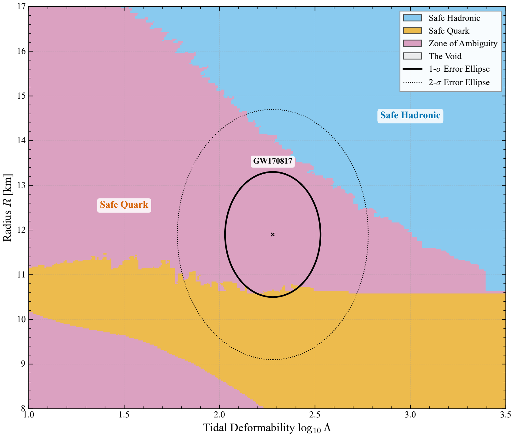
Model A: Tidal Deformability vs Radius (Ensemble)
