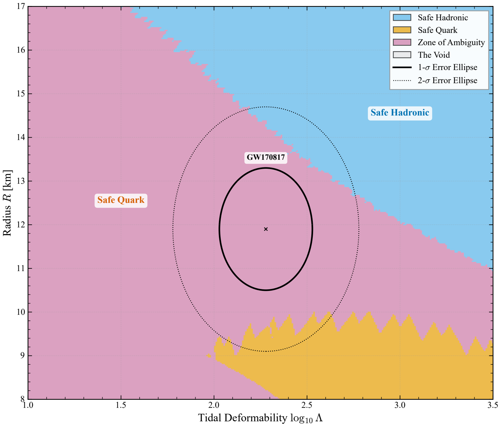
Model A: Tidal Deformability vs Radius (MLP)
