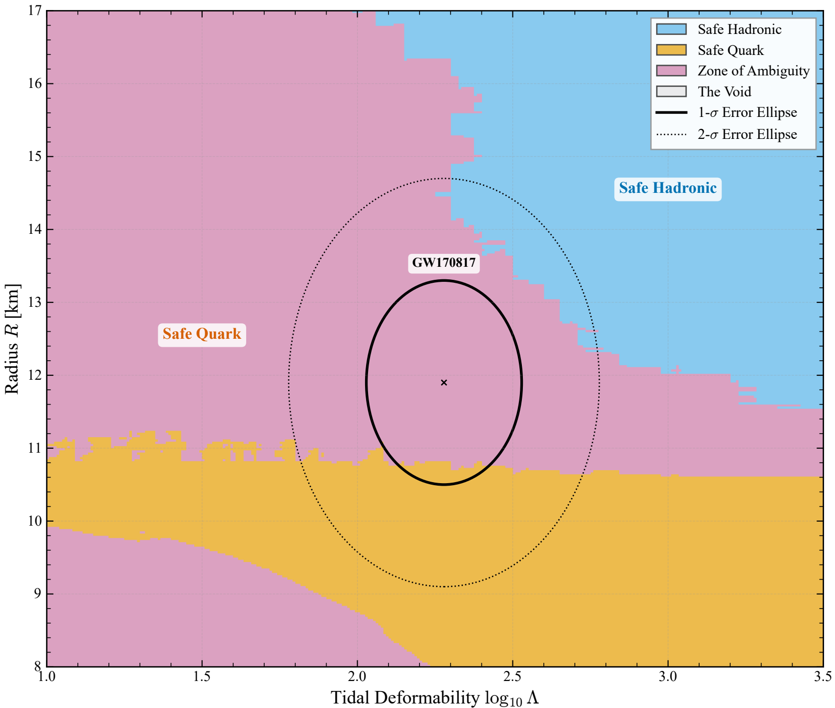
Model A: Tidal Deformability vs Radius (XGBoost)
