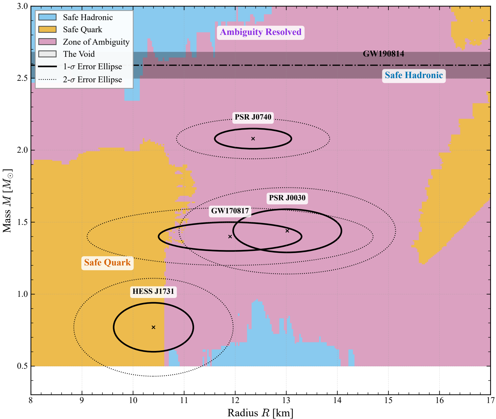
Model A: Resolving Degeneracy with \Lambda (Projected) (XGBoost)
