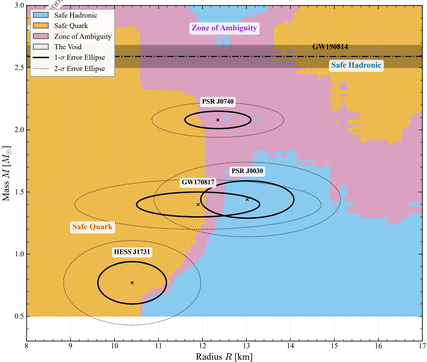
Model Geo: The Degeneracy of Mass & Radius (Ensemble)
