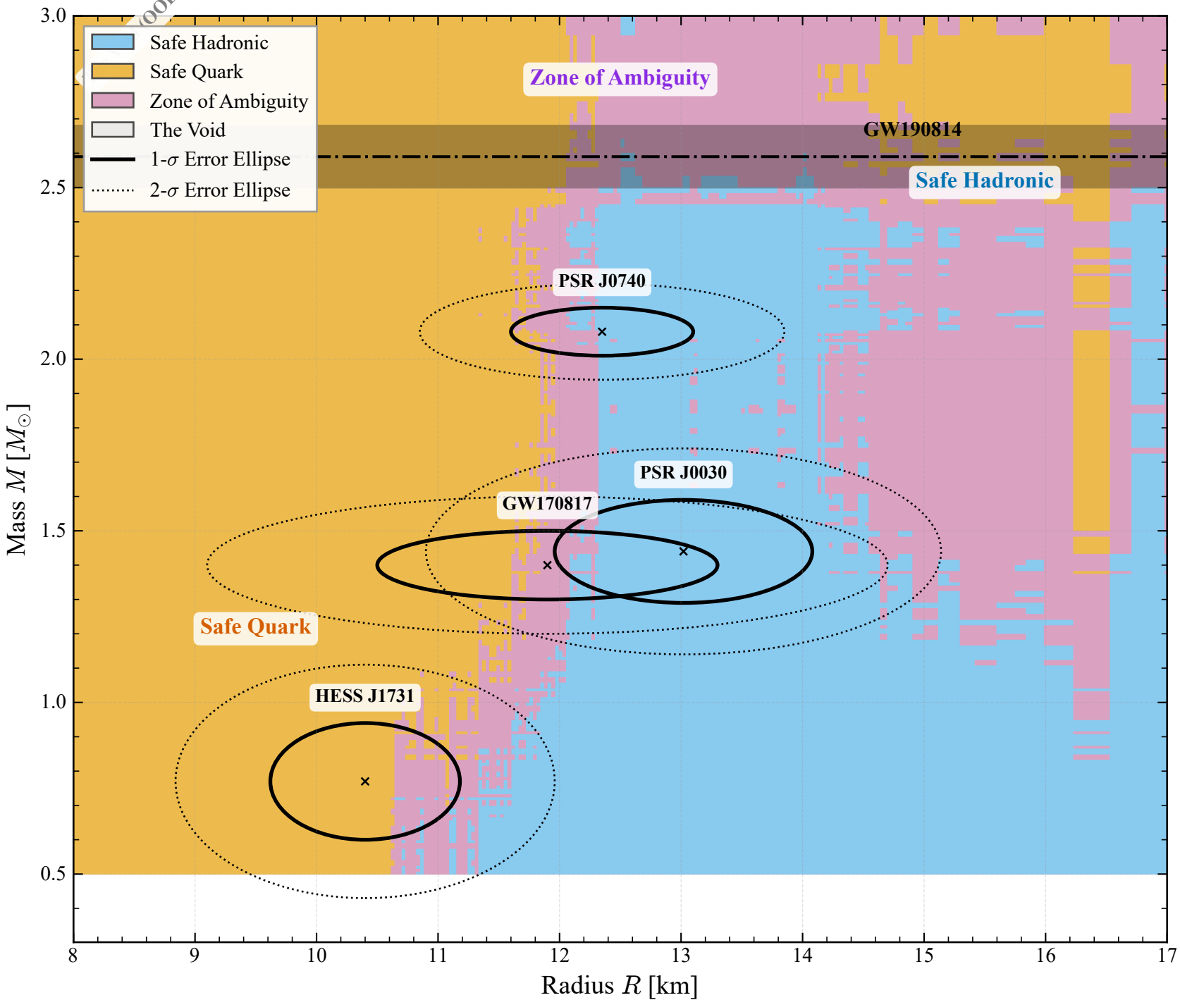
Model Geo: The Degeneracy of Mass & Radius (XGBoost)
