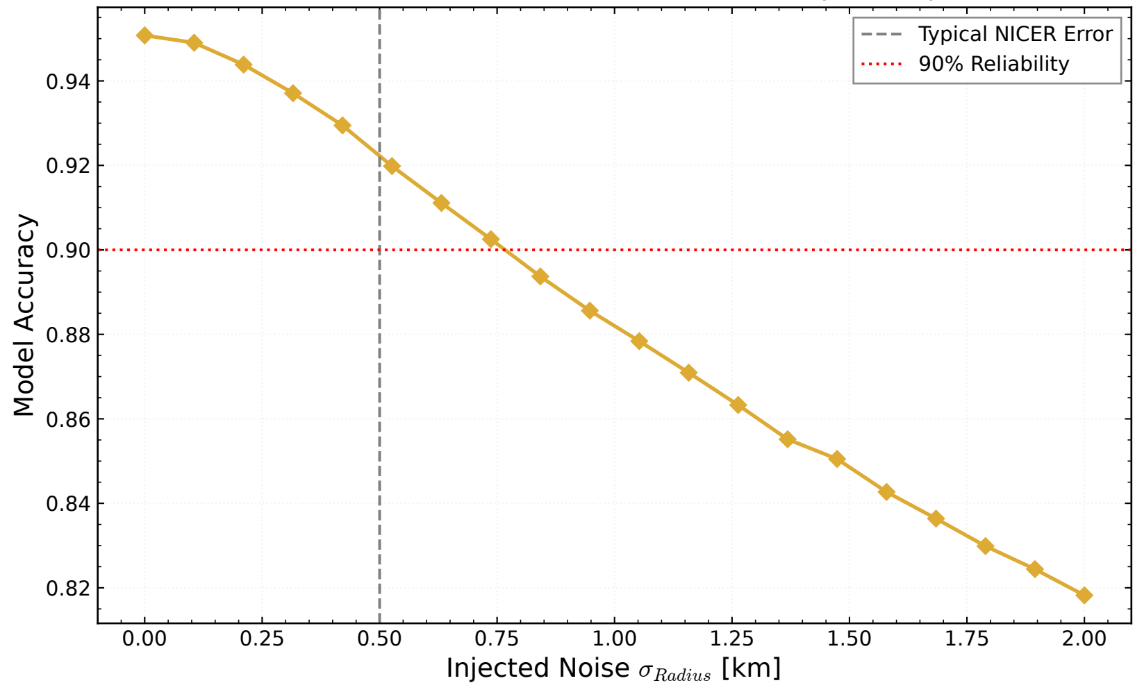
Robustness to Observational Noise (Radius)
