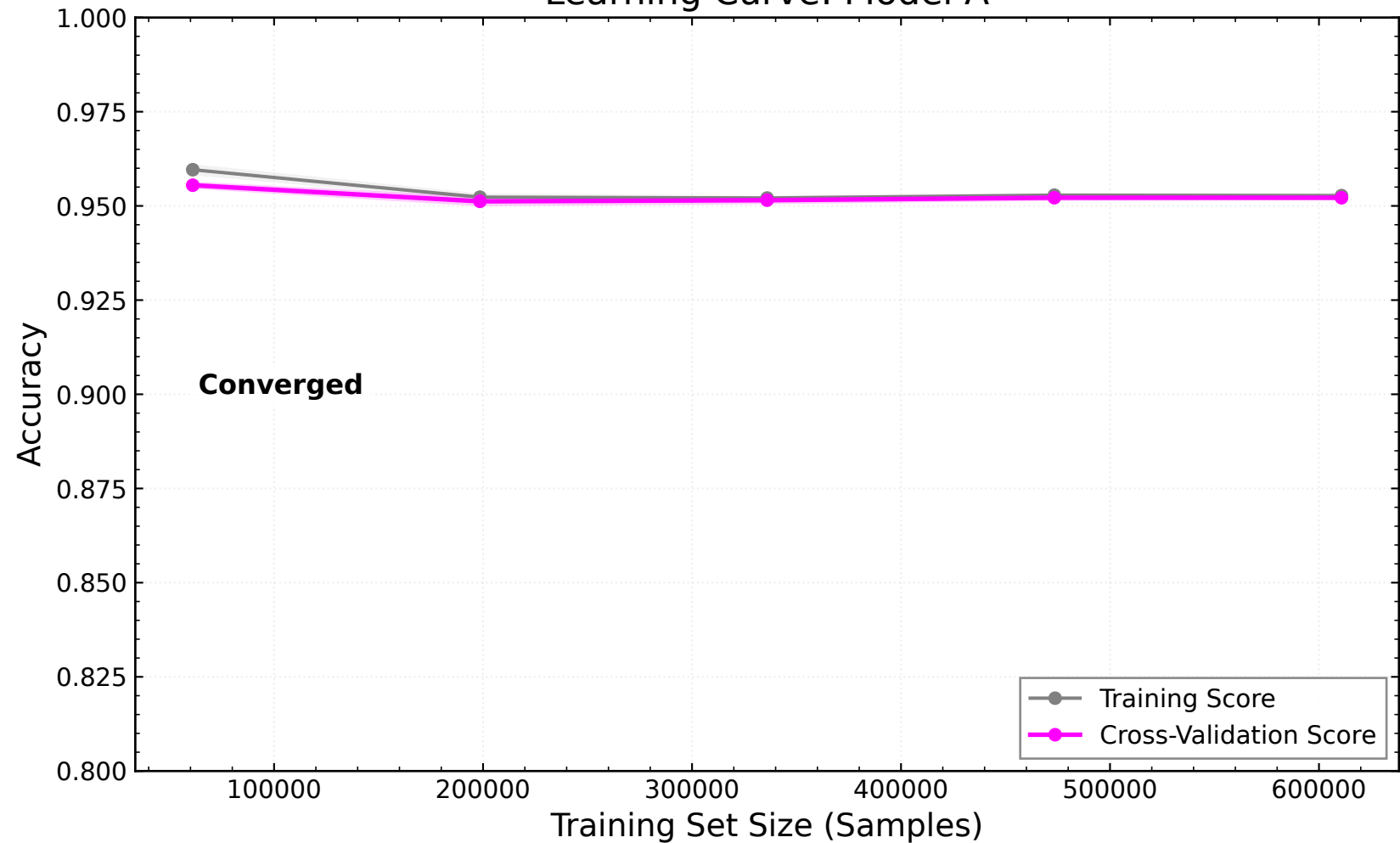
Learning Curve: Model A
