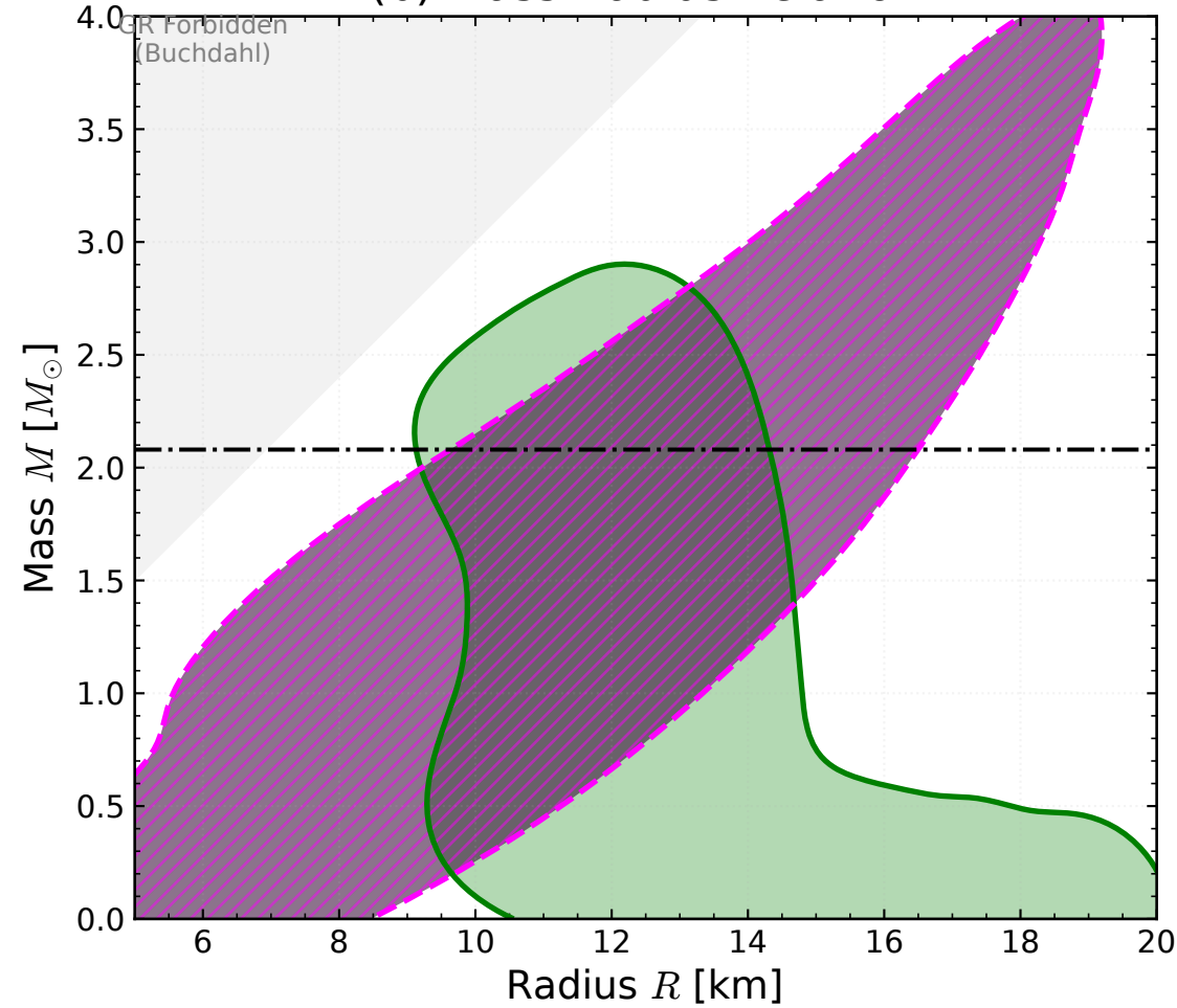
(b) Mass-Radius Relation
