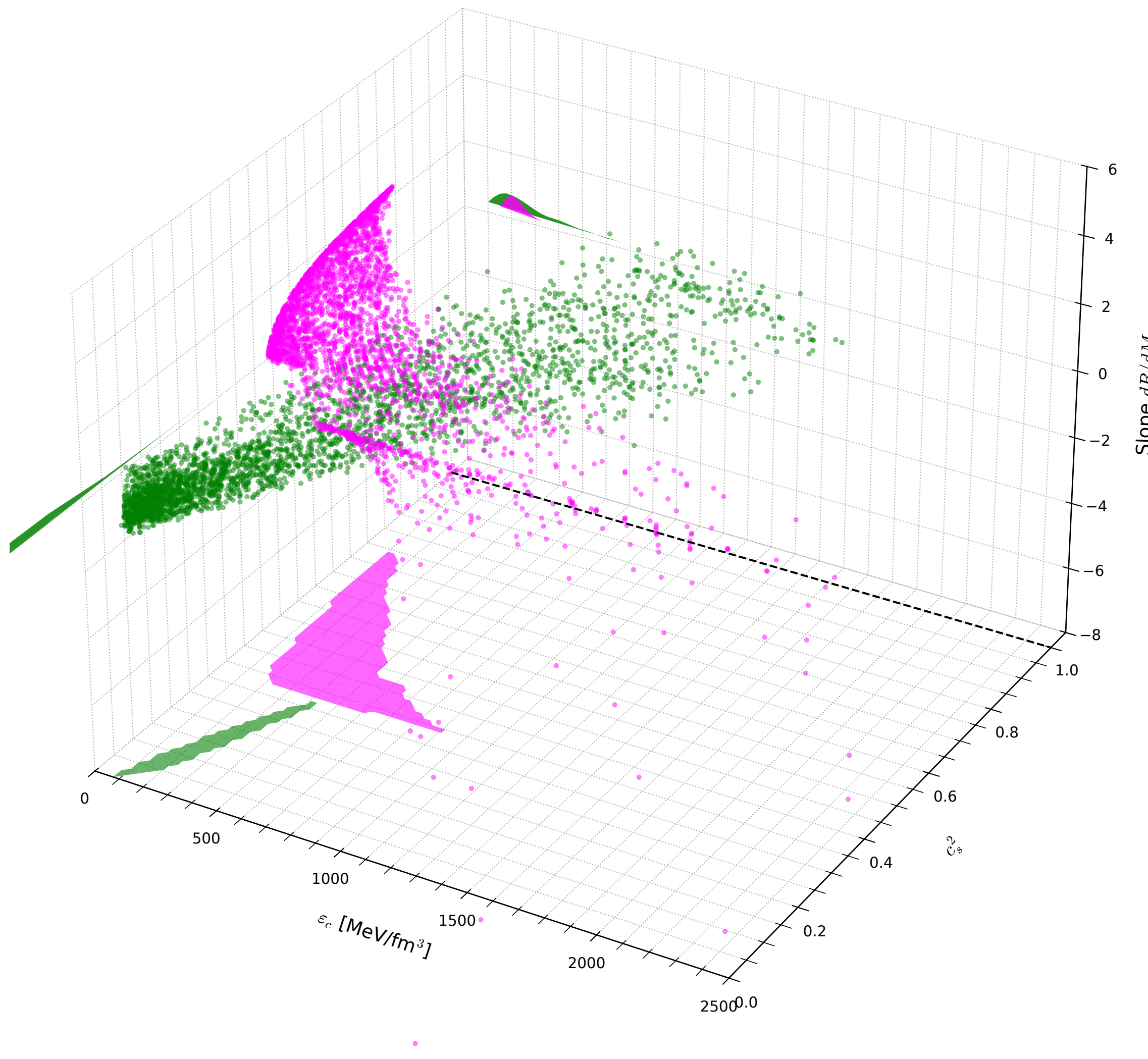
Microphysics Manifold (With Projections)
