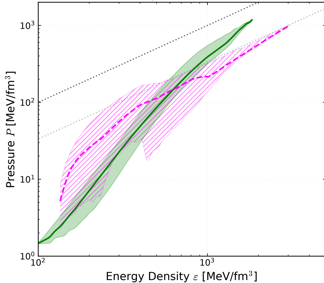
(a) Equation of State
