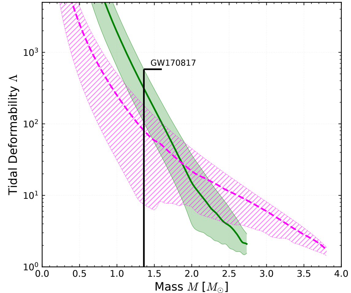
(c) Tidal Deformability
