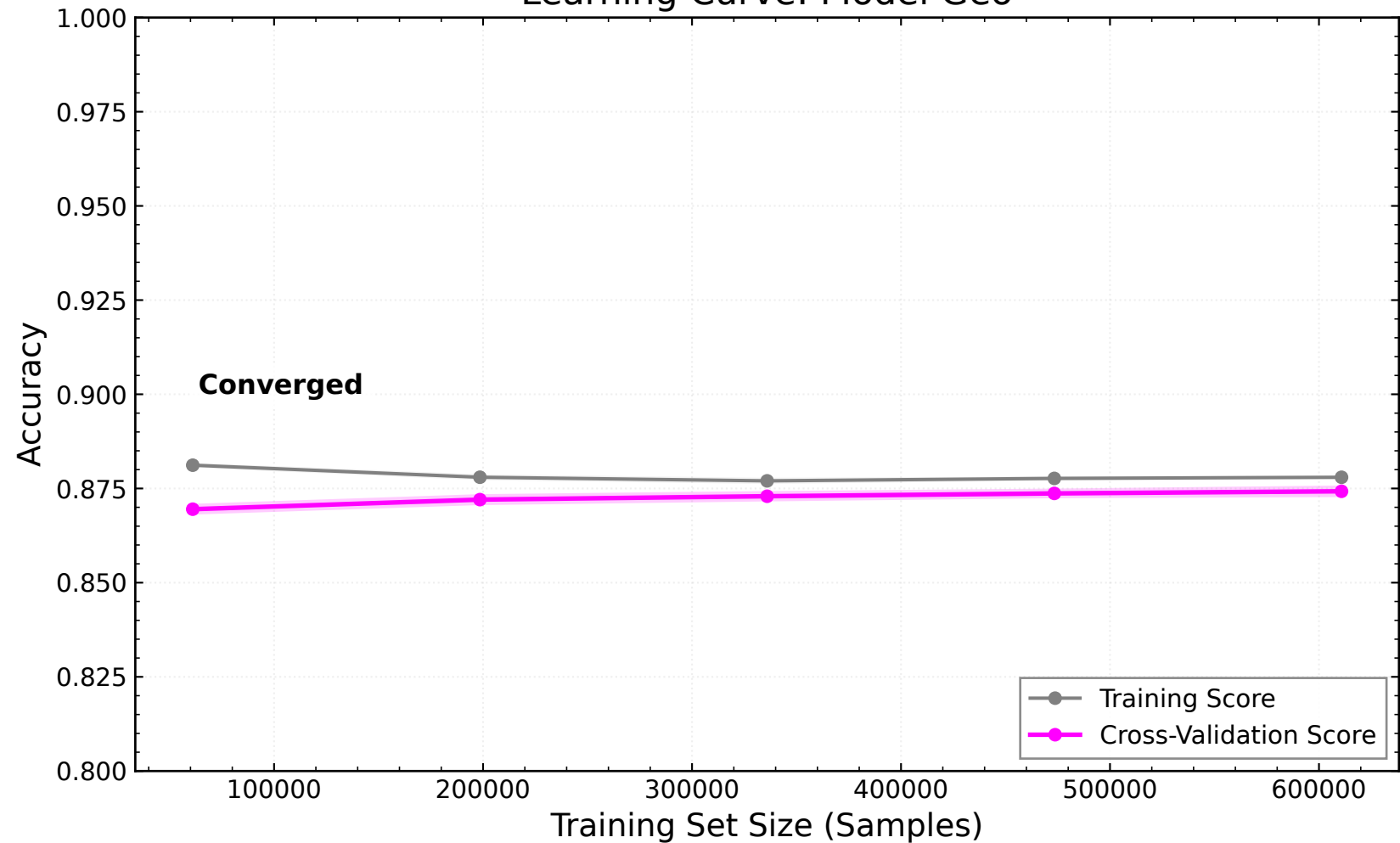
Learning Curve: Model Geo
