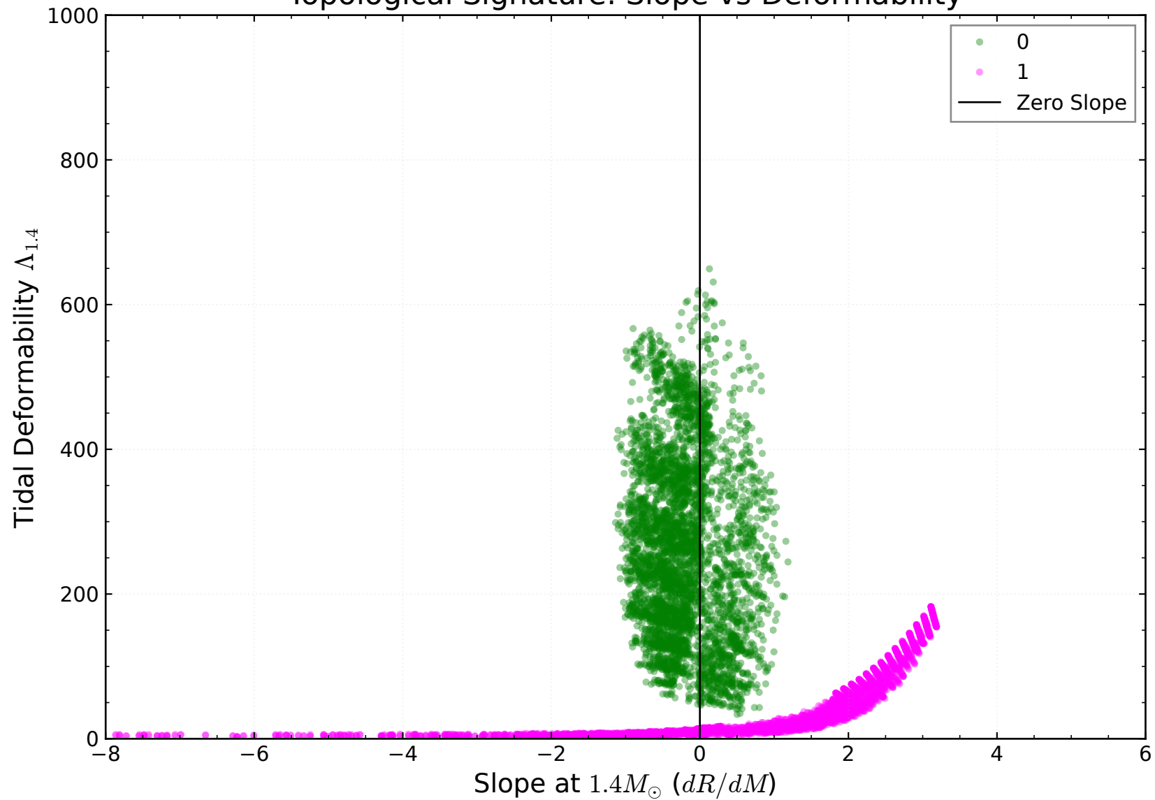
Topological Signature: Slope vs Deformability
