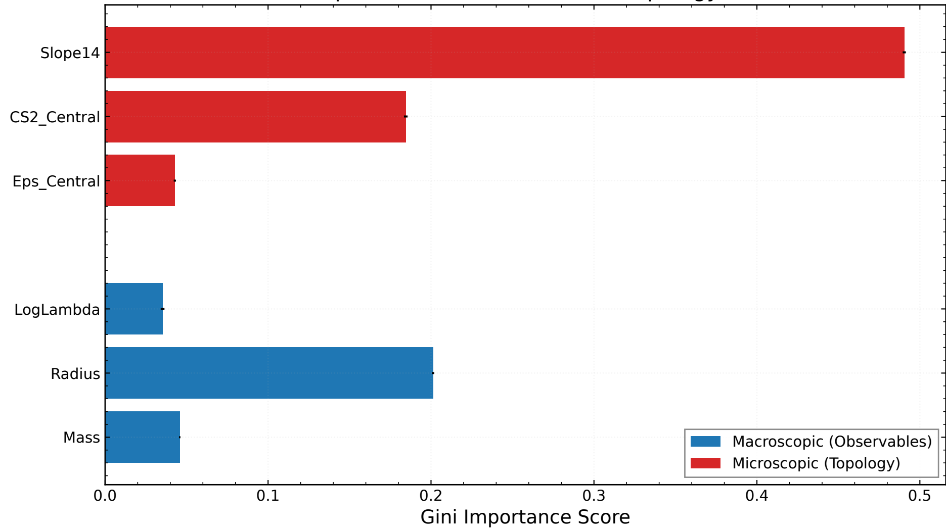
Feature Importance: Observables vs. Topology (Model D)
