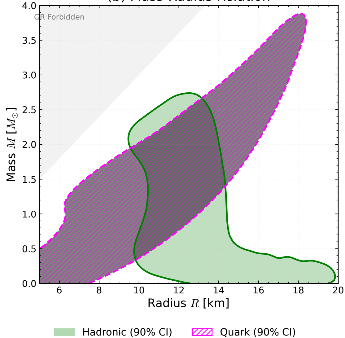
(b) Mass-Radius Relation
