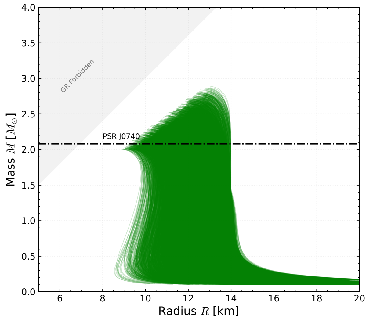
(a) Hadronic Population (All)
