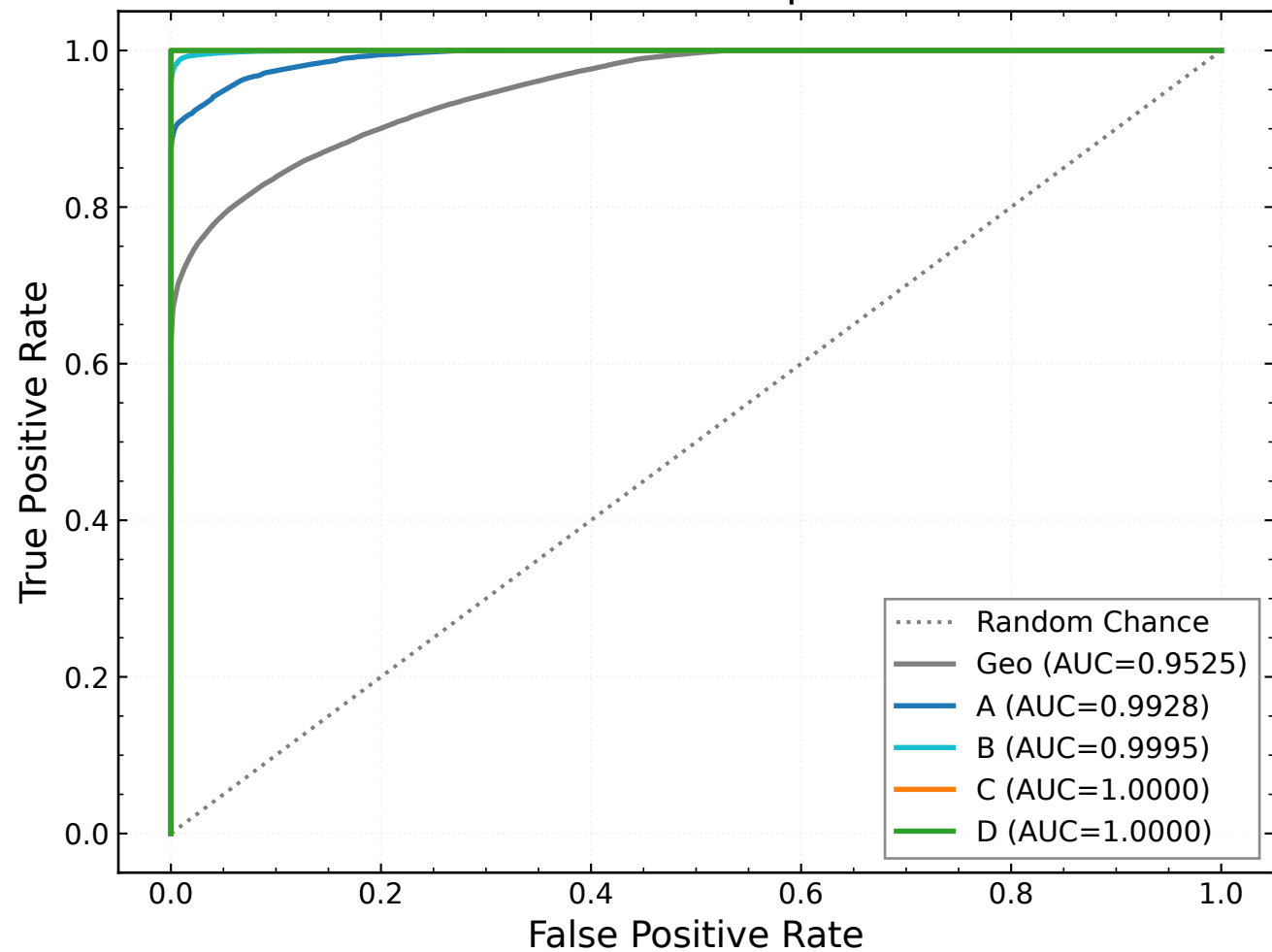
ROC Curve Comparison
