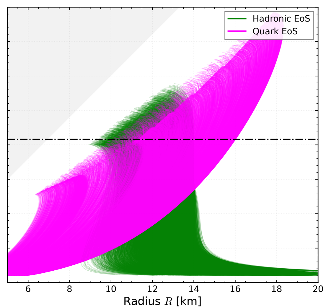
(c) Full Population Overlay
