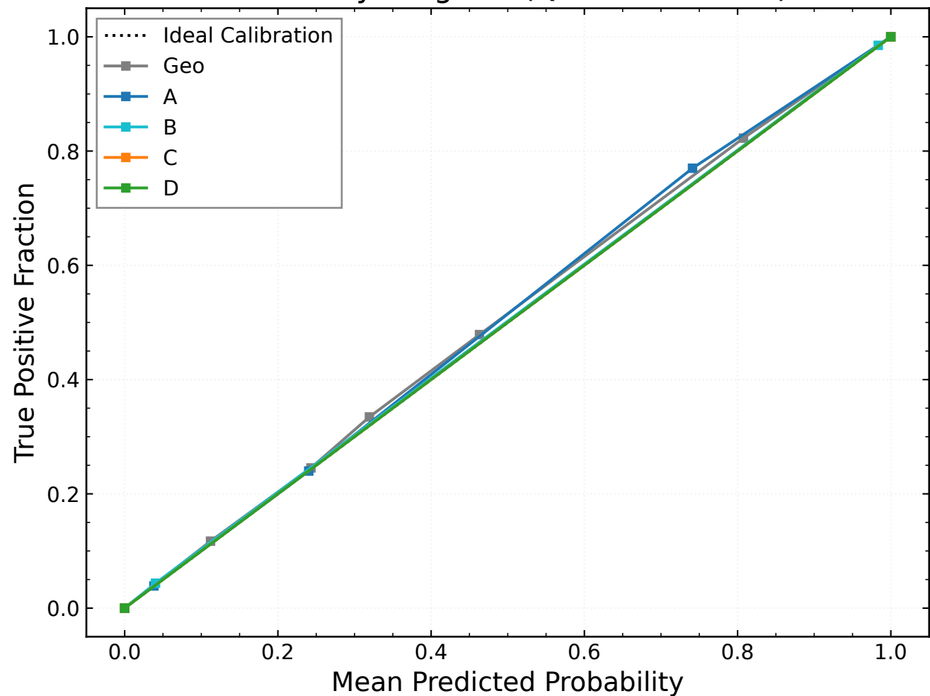
Reliability Diagram (Quantile Binned)
