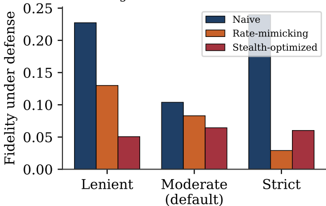
Security--utility trade-off across defense strength and attacker stealth level
