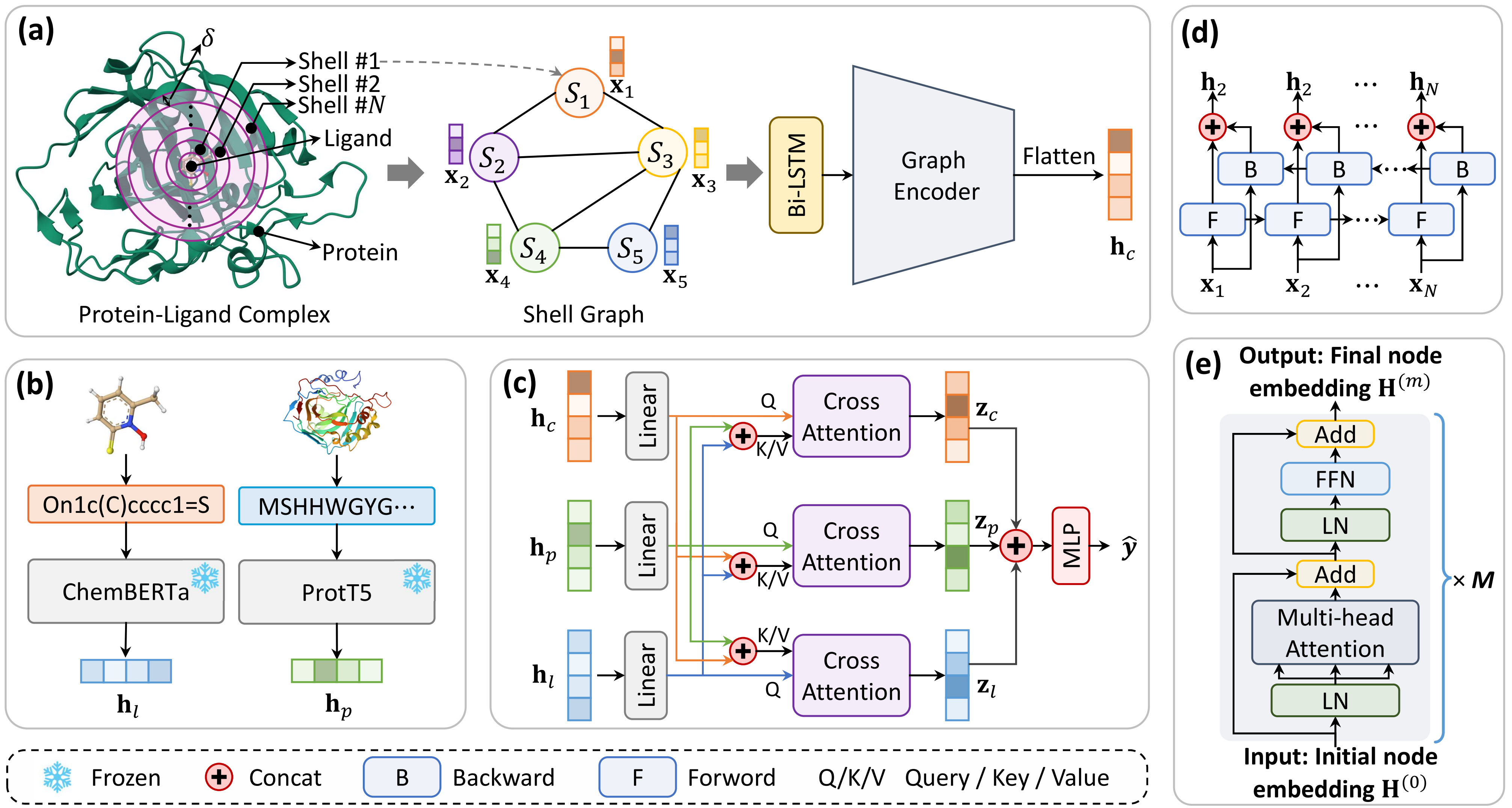
(a) Shell Graph Encoder (b) Frozen Protein-Ligand LM Encoders (c) Symmetric Tri-modal Cross-attention (d) Bi-LSTM (e) Graph Encoder
