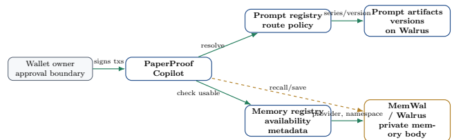
Fig. 8. Agentic interface architecture. Public registries select official prompt artifacts and memory capability metadata; private memory bodies remain in MemWal/Walrus and are accessed only through user-authorized client flows.
