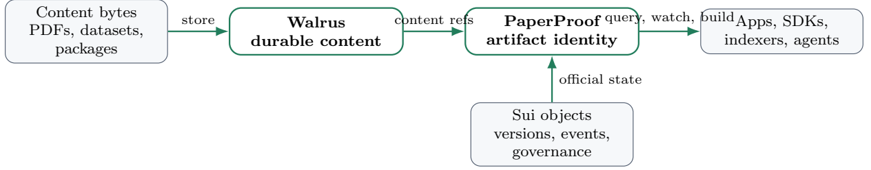
Fig. 1. PaperProof turns content stored on Walrus into Sui-native protocol artifacts with typed versions, official interactions, governance, and developer-facing query surfaces.
