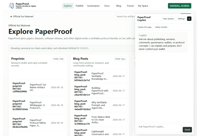
Fig. 7. PaperProof Copilot operates as a browser-side protocol guide. It can read page state and protocol-native prompts, but it remains outside the wallet authorization boundary.
