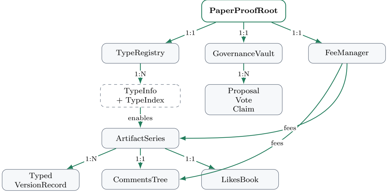
Fig. 4. PaperProof on-chain object model. The registry controls type recognition; artifact series and their official interaction objects form the durable identity surface.
