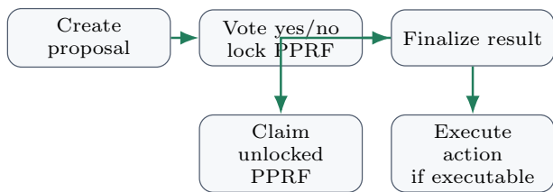
Fig. 6. PPRF governance lifecycle. Voting locks funds; finalization determines result; executable proposals may mutate protocol state; voters can claim unlocked funds according to proposal state.
