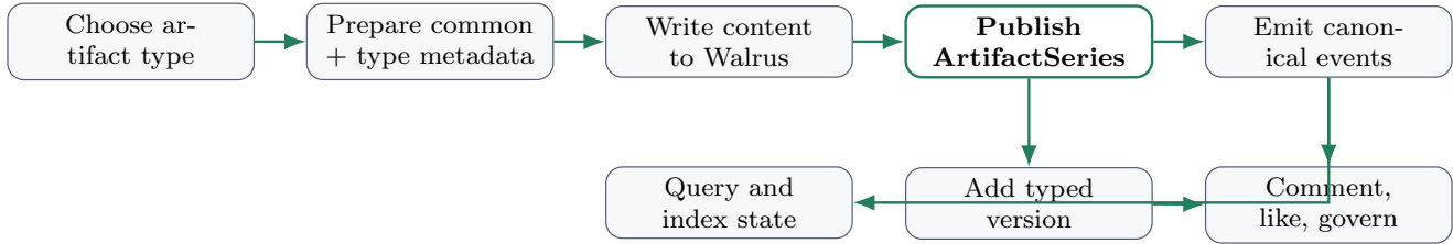
Fig. 5. Artifact lifecycle. Publication creates a series and first typed version; later versions, comments, likes, and governance actions extend the protocol life of the artifact.
