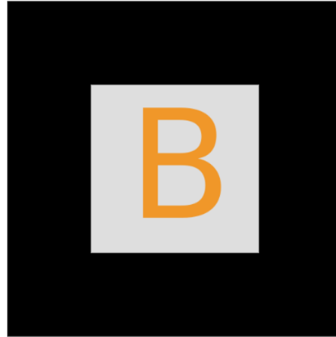
Quantum dot 2
