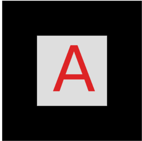
Orbital “s”
