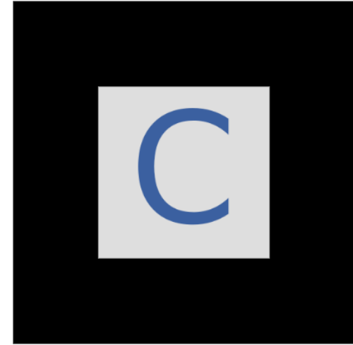
Quantum dot 3
