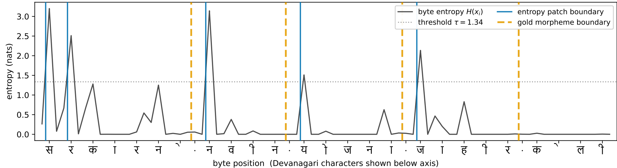
Entropy patch boundaries align with gold morpheme boundaries (neural BLT entropy model, Marathi)
