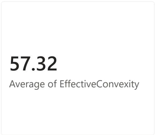
Average Convexity
