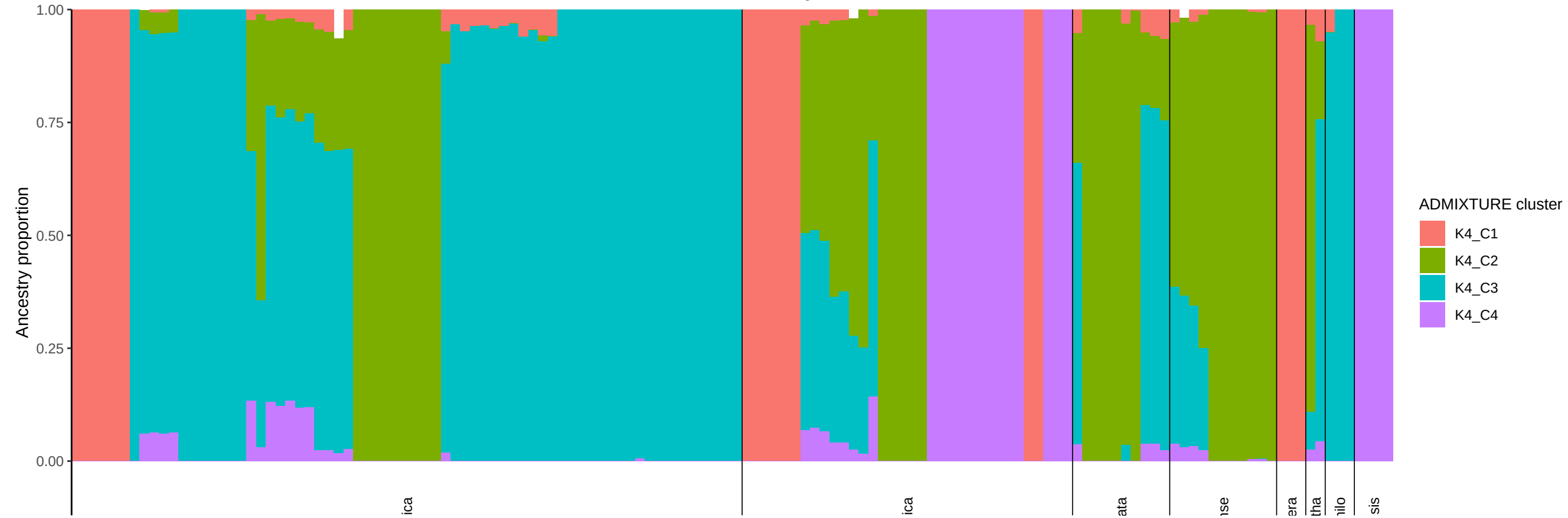
ADMIXTURE K = 4 by host
