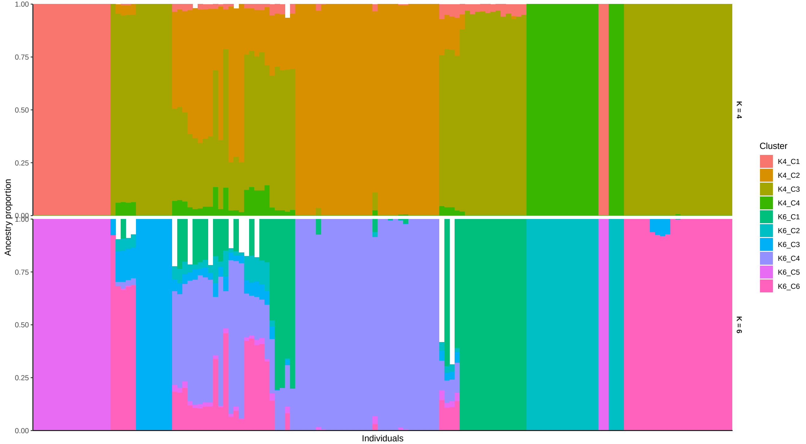
ADMIXTURE population structure
