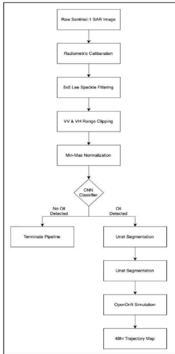
Figure 5.1: Flow Chart
