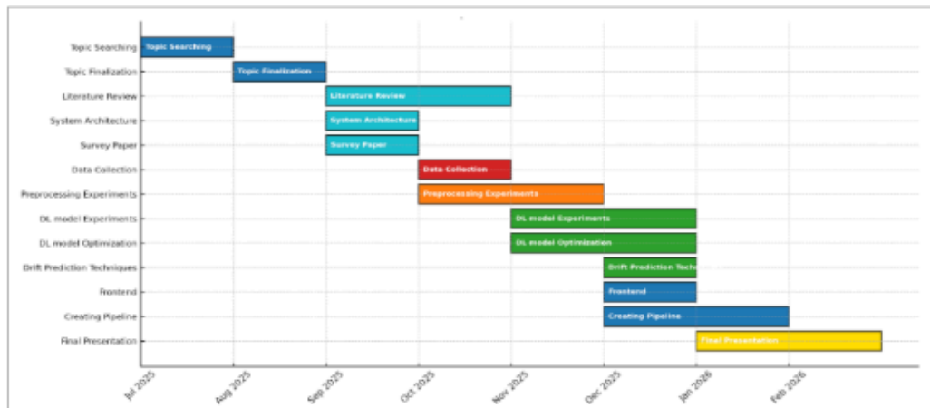
Figure 12.1: Project Plan
