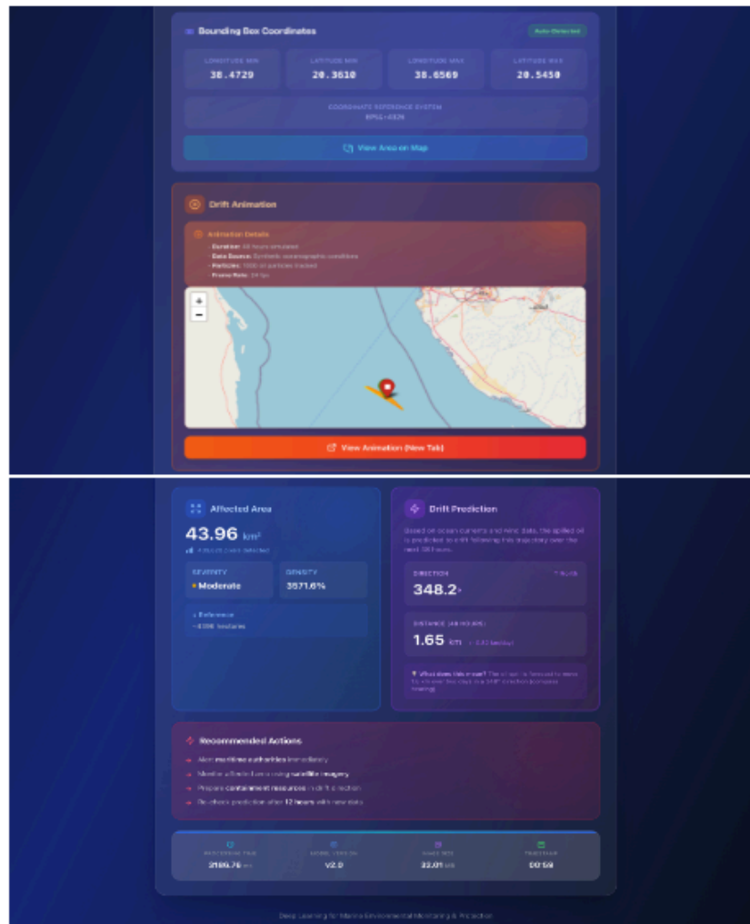
Figure 11.1: Gui Screenshots
