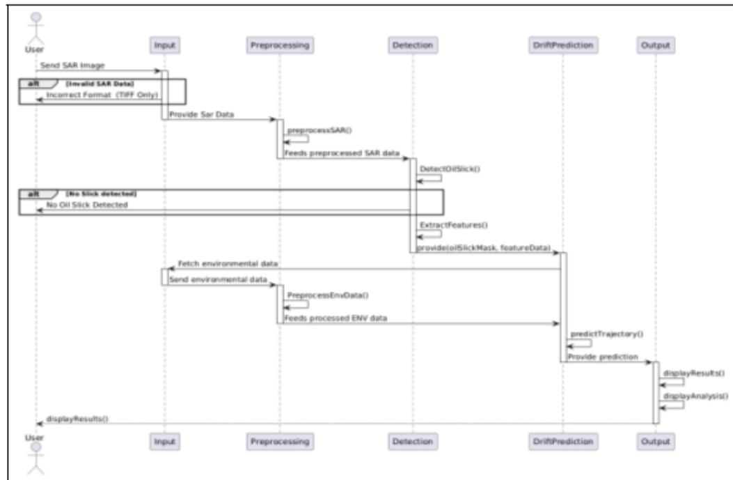
Figure 8.6: Sequence Diagram
