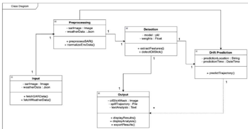
Figure 8.4: Class Diagram
