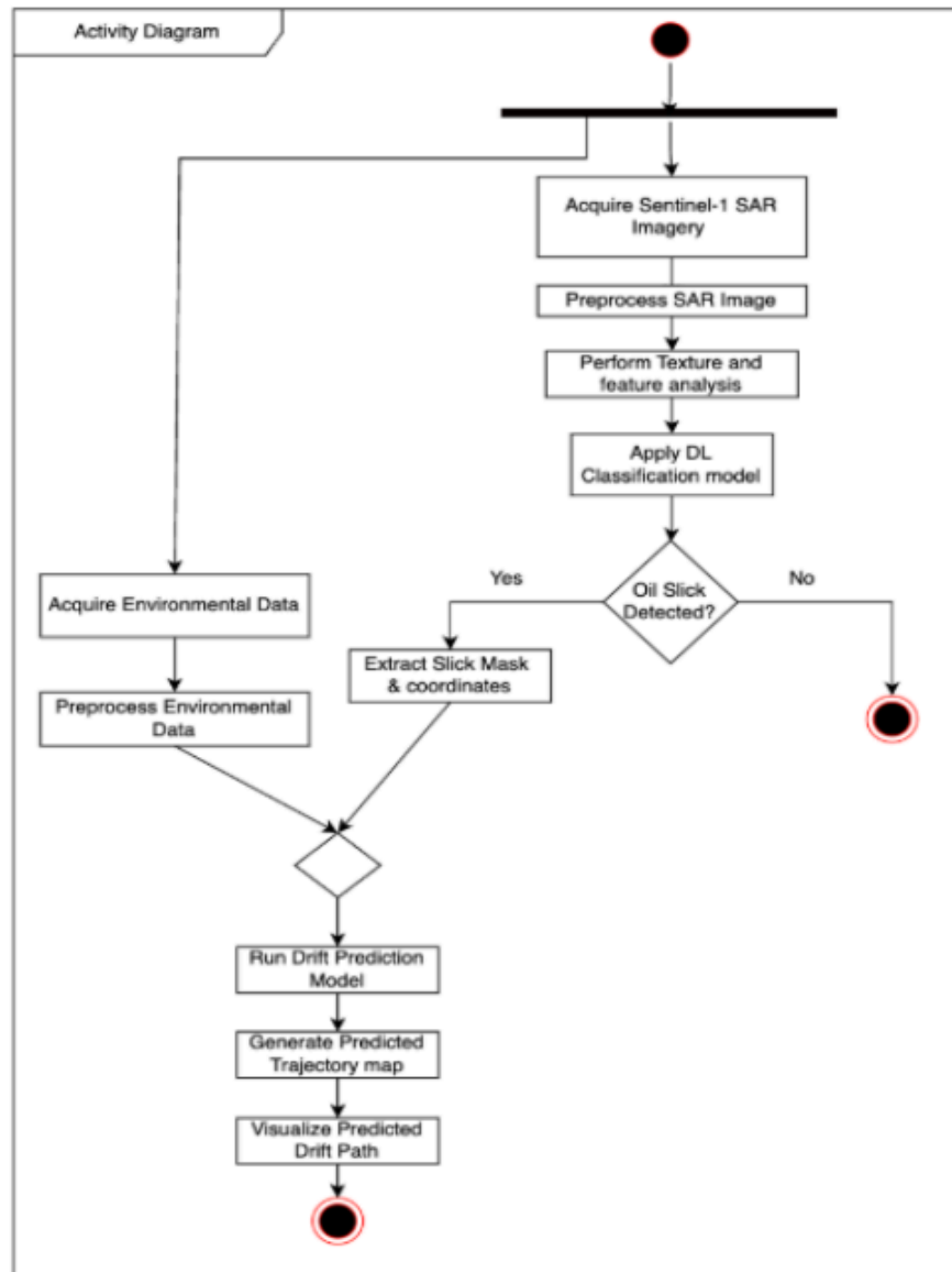
Figure 8.5: Activity Diagram
