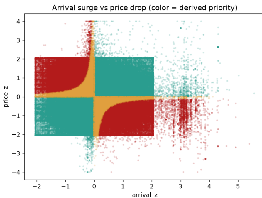
Fig 5 — Arrival surge (x) vs price drop (y), coloured by priority. Observation: High-priority points sit in the high-arrival + negative-price quadrant → validates the S = \text{arrival}_z \times (-\text{price}_z) rule.
