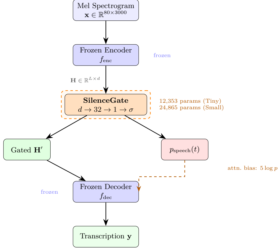
Figure 1: WhisperGate architecture. A lightweight SilenceGate MLP sits between Whisper’s frozen encoder and decoder. The gate produces per-frame speech probabilities p_{\text{speech}}(t) used for gating. Solid arrows : soft or hard multiplicative gating. Dashed arrow : attention-bias mode passes 5 \log p as cross-attention mask.
