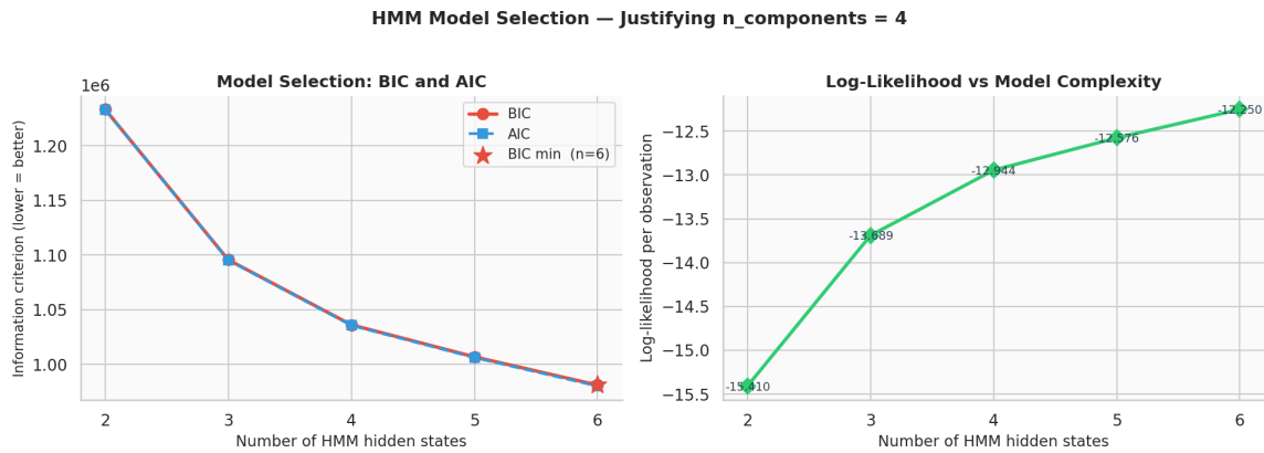
Figure 20: BIC and AIC as functions of the number of hidden states K . BIC decreases monotonically through K = 6 with no elbow at K = 4 ; the log-likelihood improvement per added component (right panel) shows no saturation. BIC-optimal: K = 6 .
