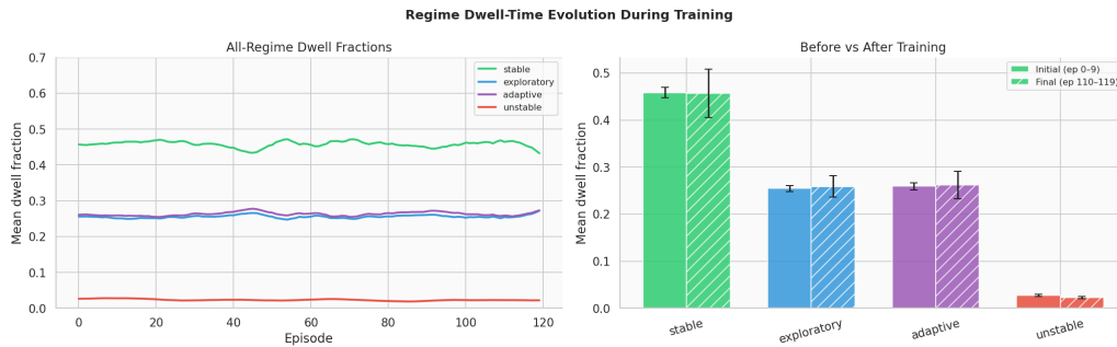
Figure 2: Regime dwell-fraction evolution across training episodes, pooled across 20 agents.
