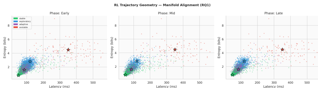
Figure 3: RL trajectory geometry in (latency, entropy) feature space across training phases (RQ1), overlaid on NB02 regime centroids.
