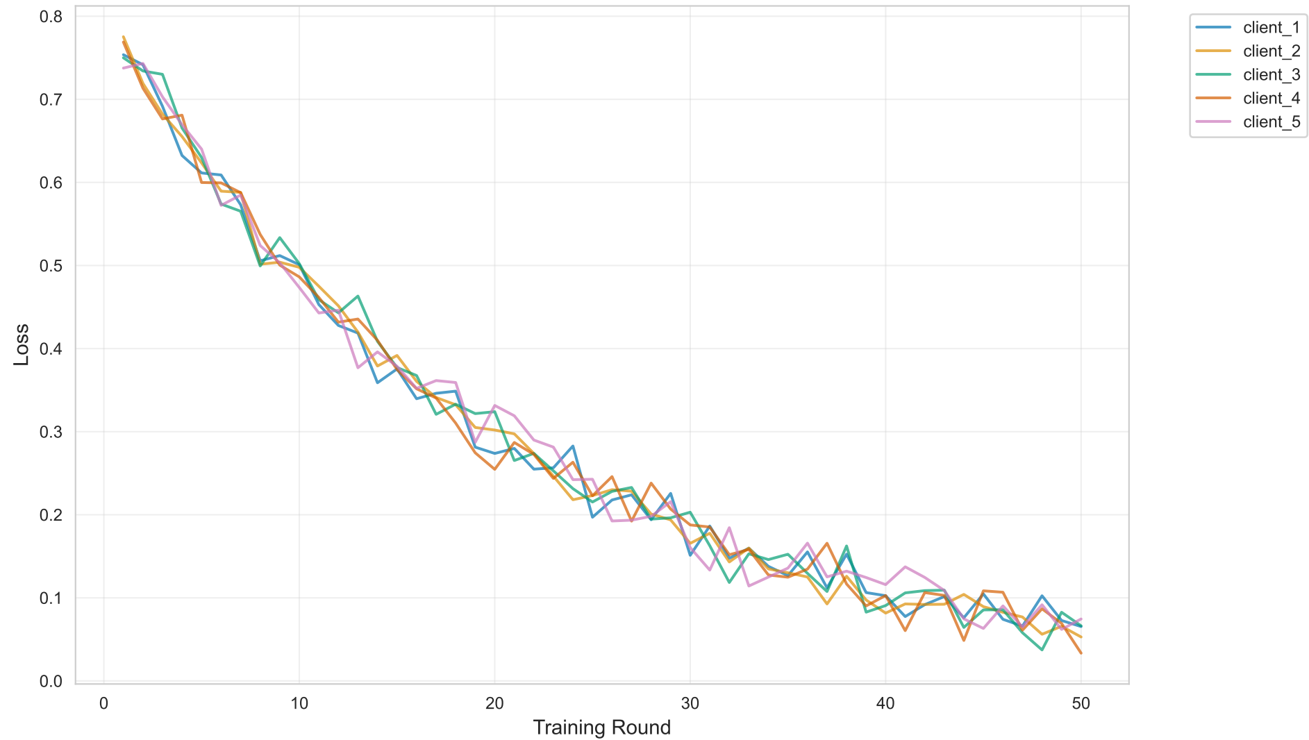
Training Loss per Client
