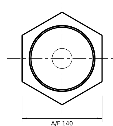
VIEW FROM ROD END (SCALE 1:4)
