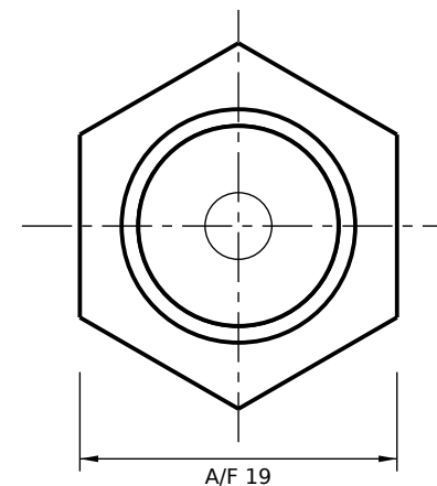
VIEW FROM ROD END (SCALE 2:1)
