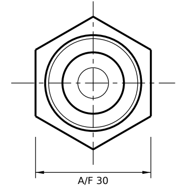
VIEW FROM ROD END (SCALE 1:1)
