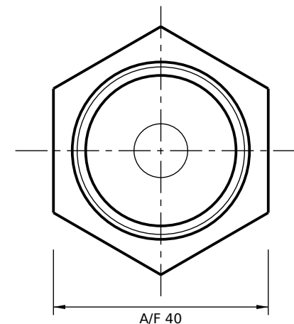
VIEW FROM ROD END (SCALE 1:1)
